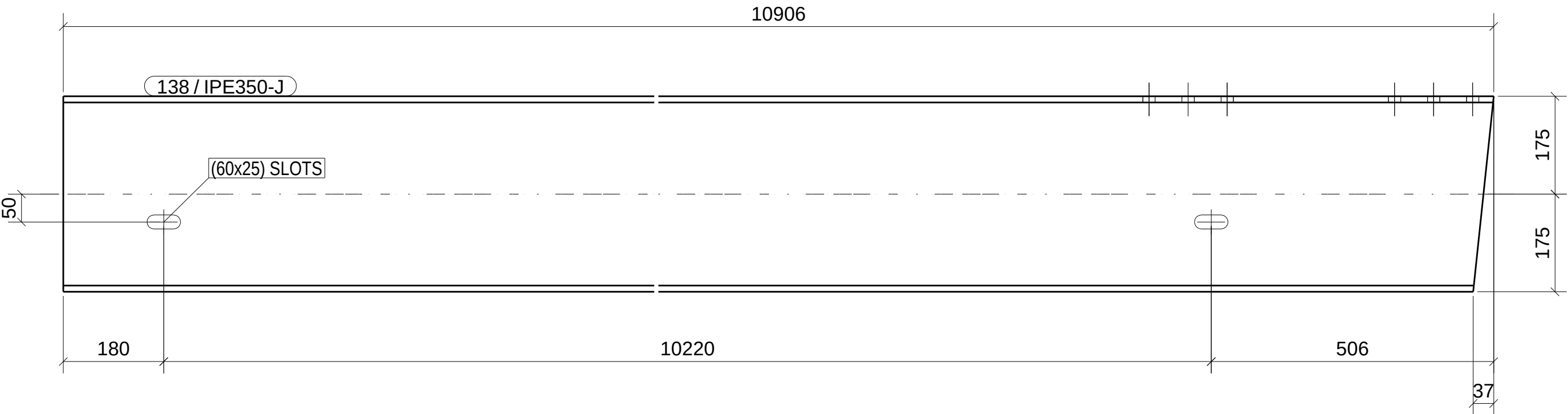
FRONT VIEW
